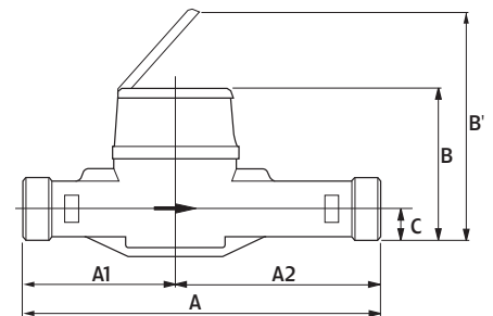
DN 15
